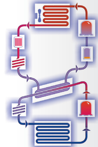
Animated Refrigeration Schematic
